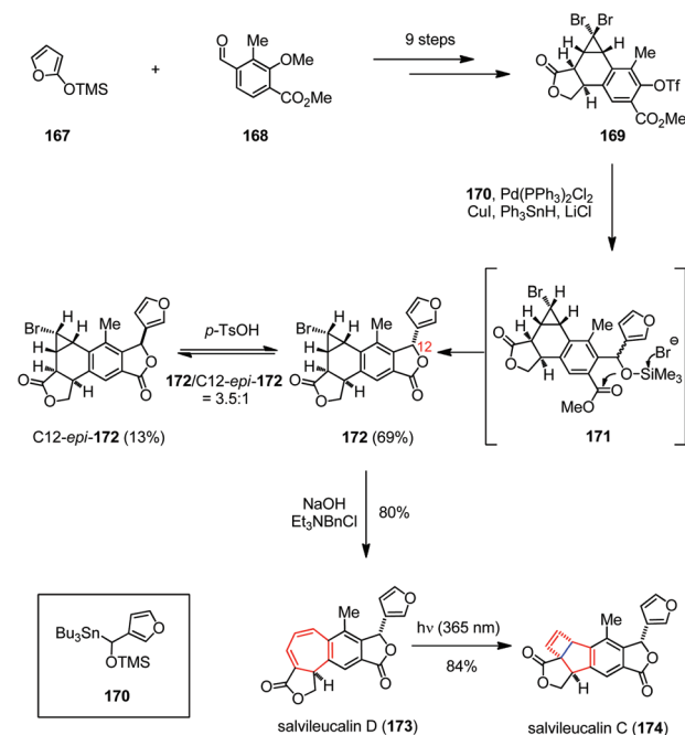
Scheme 24 4 \pi electrocyclic cyclization in the total synthesis of salvileucalin C.
