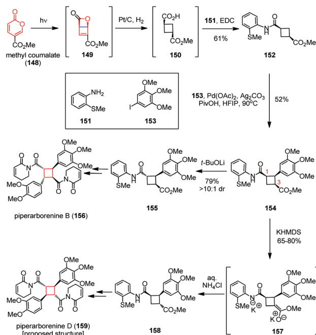
Scheme 22 4 \pi electrocyclic cyclization in the total syntheses of piperaborenines.
