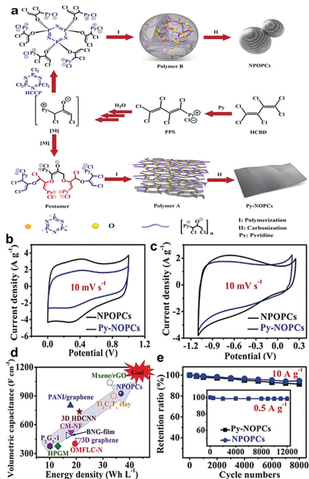
Fig. 25 (a) Proposed polymerization and carbonization route of Py-NOPCs and NPOPCs. Electrochemical evaluation of Py-NOPCs and NPOPCs: cyclic voltammety (CV) tests at 10 mV s -1 in the first cycle, in 0.5 m H 2 SO 4 (Py-NOPCs) (b) and 6 m KOH (NPOPCs) (c). (d) Volumetric specific capacitance vs. energy density for different materials. (e) Cycling performance of NPOPCs in 6 m KOH at a current density of 10 A g -1 (inset: cycling performance at a current density of 0.5 A g -1 ). Reproduced with permission from ref. 172. Copyright 2019 Wiley-VCH Verlag GmbH & Co. KGaA, Weinheim.
