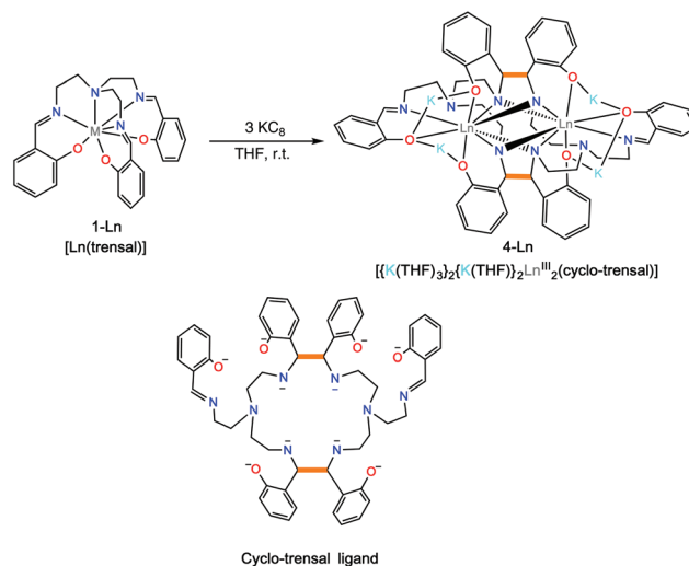
Scheme 4 Synthesis of [\{K(THF)_3\}_2(K(THF)_2)Ln_2(cyclo-trensalcone)] , 4-Ln , Ln = Nd, Sm.
