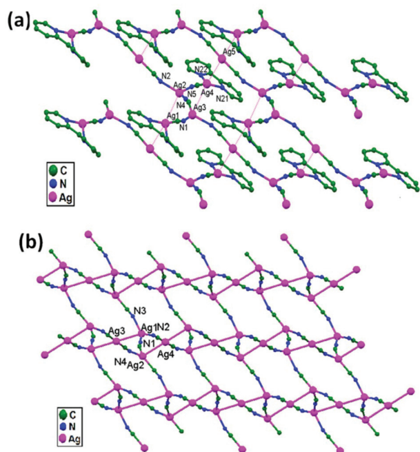
Fig. 29 Ligand-unsupported argentophilic interactions forming 2D networks in (a) compound 47 and (b) compound 48.
