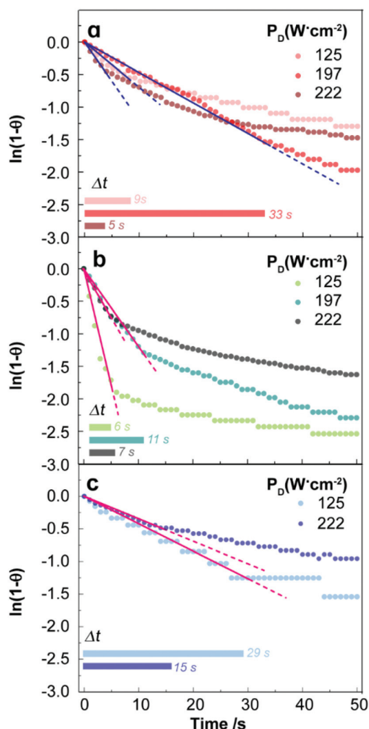
Fig. 2 Time-dependence of the reduced temperature for the (a) uncapped UCNPs and (b) lipid bilayer-capped UCNPs dispersed in \text{H}_2\text{O} , and (c) uncapped UCNPs dispersed in \text{D}_2\text{O} , measured by the immersed thermocouple. The logarithmic representation of the reduced temperature profiles allows the identification of the time range in which \ln[1 - \theta(t)] is linear. The horizontal bars mark the time interval ( \Delta t ) in which these linear fits are verified. The solid lines are the best fits to eqn (16) ( r^2 > 0.970 ) and the dashed lines are guides for the eyes.
