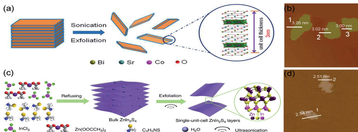
Fig. 2 Schematic illustration of ultrasonic exfoliation of bulk (a) BCSO and (c) \text{ZnIn}_2\text{S}_4 ; AFM images of single-unit-cell (b) BCSO and (d) \text{ZnIn}_2\text{S}_4 . (a and b) Reproduced from ref. 5. Copyright 2018, American Chemical Society. (c and d) Reproduced from ref. 61. Copyright 2017, Springer Nature.
