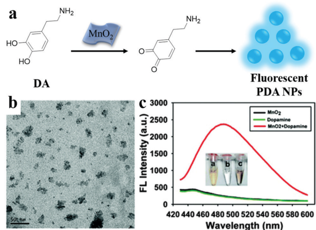
Fig. 9 (a) Schematic illustration of the synthesis of fluorescent PDA NPs. (b) TEM image of the fluorescent PDA NPs. (c) Fluorescence emission spectra of dopamine, \text{MnO}_2 , and the mixture of dopamine and \text{MnO}_2 . 59 Reproduced from ref. 59 with permission from the Royal Society of Chemistry.
