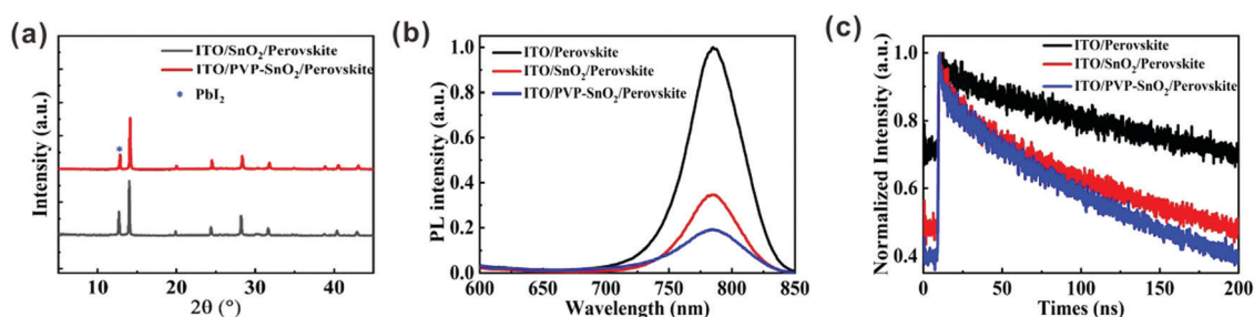
Fig. 4 (a) X-ray diffraction (XRD) patterns of the perovskites deposited on different ETLs. (b) Photoluminescence (PL) spectra of the perovskite films deposited on ITO, SnO 2 and PVP-SnO 2 substrates. (c) Normalized time-resolved photoluminescence (TRPL) spectra of the perovskite films deposited on ITO, SnO 2 and PVP-SnO 2 substrates.
