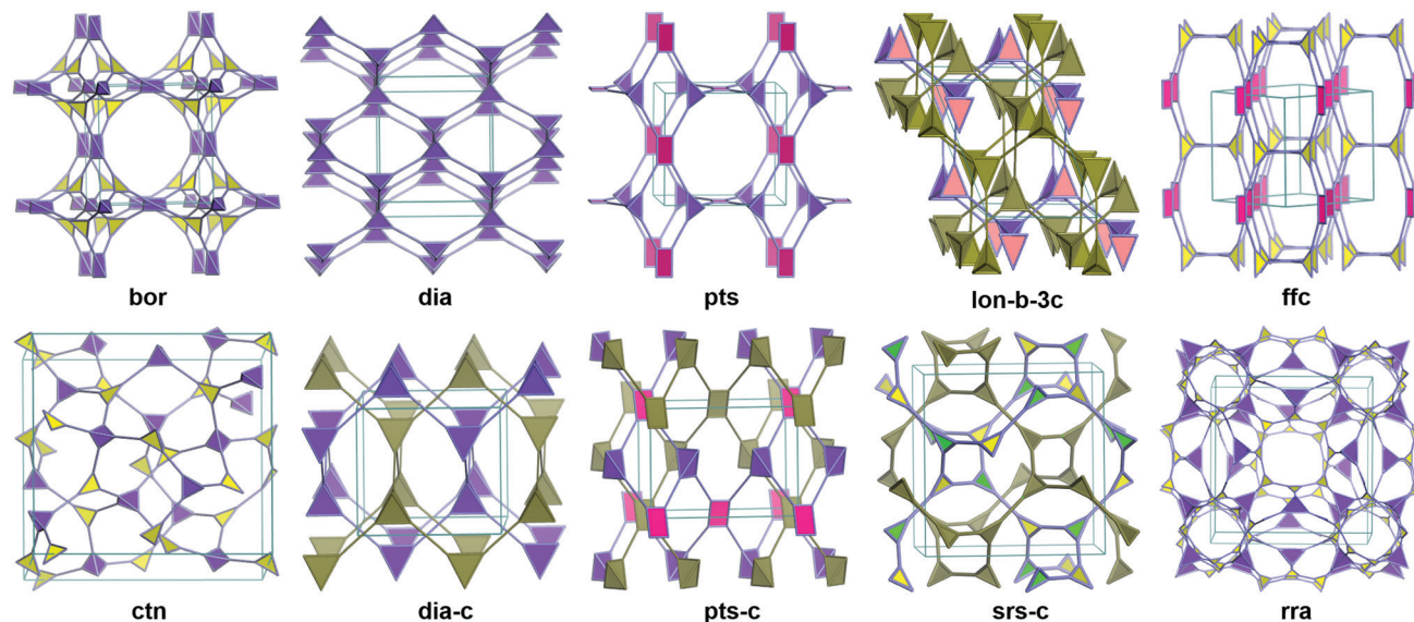
Fig. 1 Topologies in 3D COFs.
