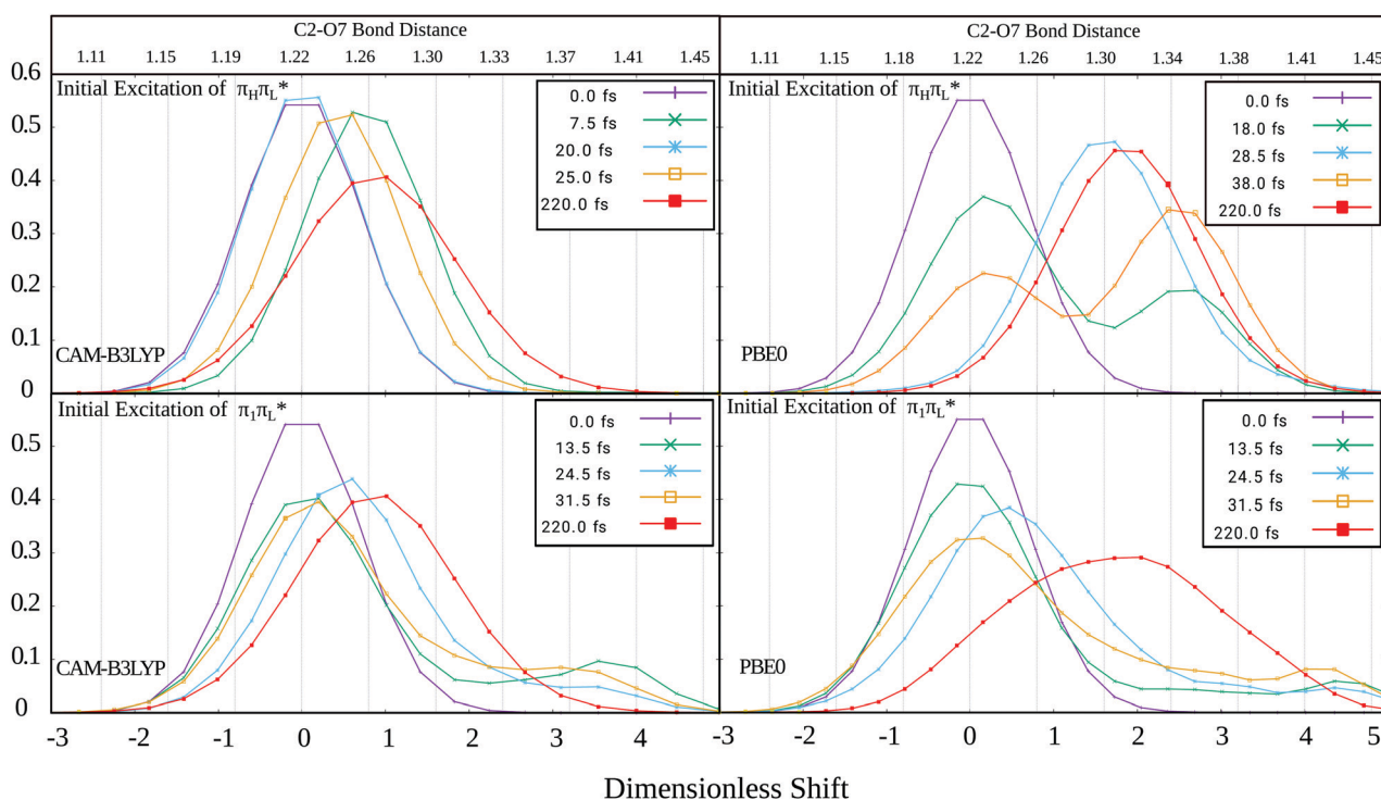
Fig. 5 Reduced density of the wavepacket along normal mode 42 (i.e. integrated along all other coordinates) at different times after the photoexcitation of \pi_H\pi_L^* (top) and \pi_L\pi_L^* (bottom), obtained by LVC Hamiltonians parameterized with CAM-B3LYP (left) or PBE0 (right). The inset shows the C2–O7 bond distances in angstroms for different dimensionless shifts of mode 42.
