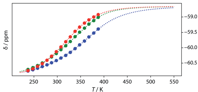
Fig. 11 ^{19}\text{F} NMR (500 MHz, TCE- \text{d}_2 , 7.4 mM) melting experiments. The lines show fitting of a two-state equilibrium isochore to the AD data (red) and a three-state isochore to the ADAD data (inner residue green, outer residue blue).
