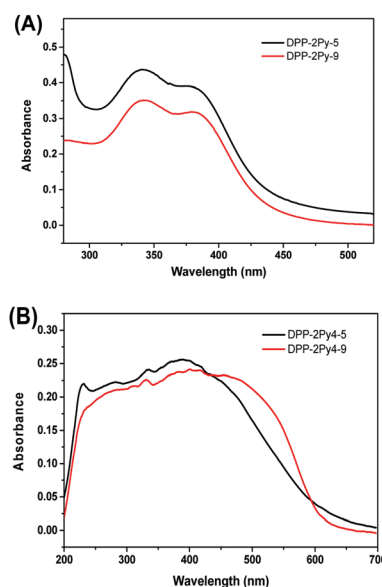
Fig. 1 The absorption spectra of DPP-2Py-5 and DPP-2Py-9 in THF solutions ( 10^{-5}\text{ M} ) (A) and solid states (B).
