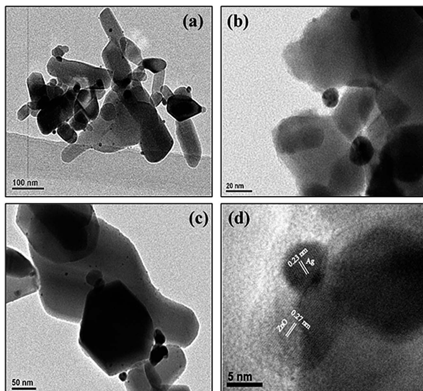
Fig. 3 TEM images (a and b) for 1 wt% Ag-ZnO and (c and d) 3 wt% Ag-ZnO.
