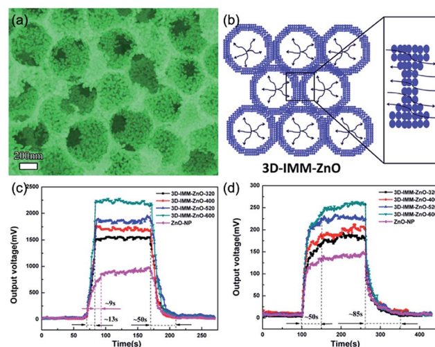
Fig. 12 (a) Morphology of 3D interconnected macro-mesoporous ZnO (3D-IMM-ZnO) nanostructure. (b) Schematic illustration of 3D-IMM-ZnO for gas sensing. Response and recovery time curves of 3D-IMM-ZnO nanostructures to (c) 100 ppm acetone at 260 °C and (d) 100 ppm methanol at 240 °C. Reproduced with permission. 130 Copyright 2016, American Chemical Society.
