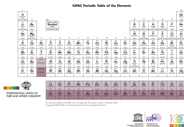
Fig. 1 The modern medium length form of the periodic table ( https://iupac.org/wp-content/uploads/2018/12/IUPAC_Periodic_Table-01Dec18.jpg ).
