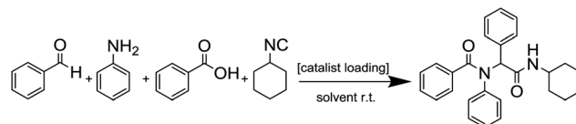
Scheme 2 Ugi reaction combination of benzaldehyde, aniline, benzoic acid and cyclohexyl isocyanide.
