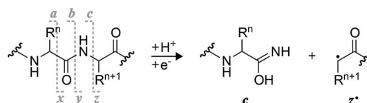
Scheme 1 Complementary c and z • fragments from N–Cα backbone bond cleavage between residues n and n + 1 in ECD, niECD, or ETD; z • fragment structures were confirmed by infrared ion spectroscopy, 22 c fragments with imidic acid structure can tautomerize to the amide form, 23 and H + transferring from a c to its complementary z • fragment can produce a pair of complementary c • and z fragments. 24,25
