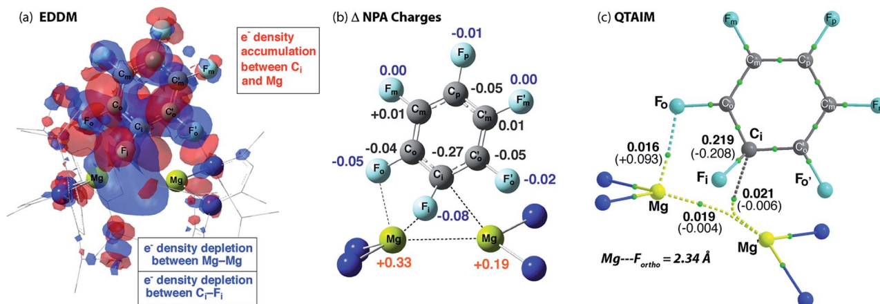
Fig. 4 (a) Energy density difference map (EDDM) for TS-1 , (b) the change ( \Delta ) in NPA charges from Int-A' to TS-1 and (c) QTAIM data on TS-1 : \rho_{(r)} values in bold, \nabla^2\rho values in parentheses. Full QTAIM for TS-1 in Fig. S28b †
