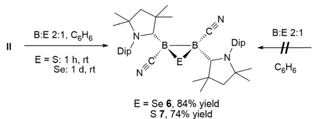
Scheme 5 Direct synthesis of 1,2,3-chalcogenadiboriranes from 2 only.
