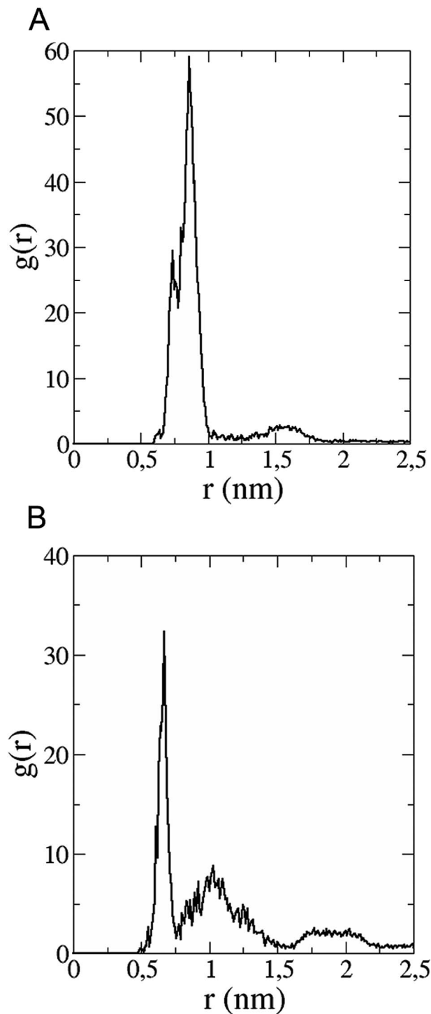
Fig. 8 (A) Radial distribution function versus distance of 5R residue (A \beta 42 ) between centres of mass of residue and fullerene trisadduct. (B) Radial distribution function as a function of the distance between the centre of mass of 1D residue and the two oxygen atoms in the COO-group.
