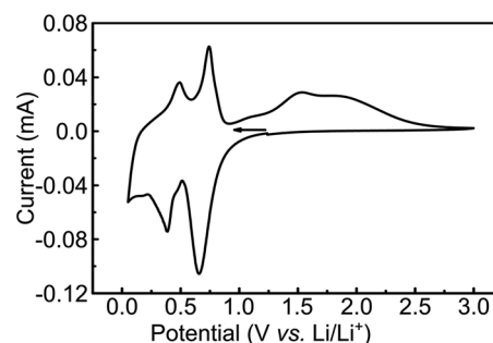
Fig. 7 Cyclic voltammetry of \text{MoS}_2 -NR films in ITO at 0.05 \text{ mV s}^{-1} scan rate. Electrolytic solution: 1 \text{ mol L}^{-1} \text{ LiTFSI} in PC.
