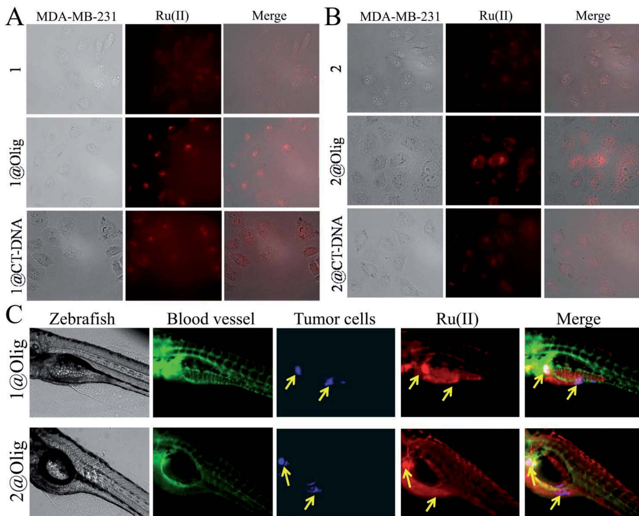
Fig. 6 Selectively imaging tumor cells by \text{Ru(II)}@ oligonucleotide in vitro and in vivo . (A) MDA-MB-231 cells imaging of 1 , 1@oligonucleotide and 1@CT-DNA at 37^\circ\text{C} for 24 h. (B) MDA-MB-231 cells imaging of 2 , 2@oligonucleotide and 2@CT-DNA at 37^\circ\text{C} for 24 h. (C) Tumor area highlighted by 1@oligonucleotide and 2@oligonucleotide in zebrafish xenografts model. ( [\text{Ru}] = 2.5 \mu\text{M} , [\text{oligonucleotides}] = 2.5 \mu\text{M} ).
