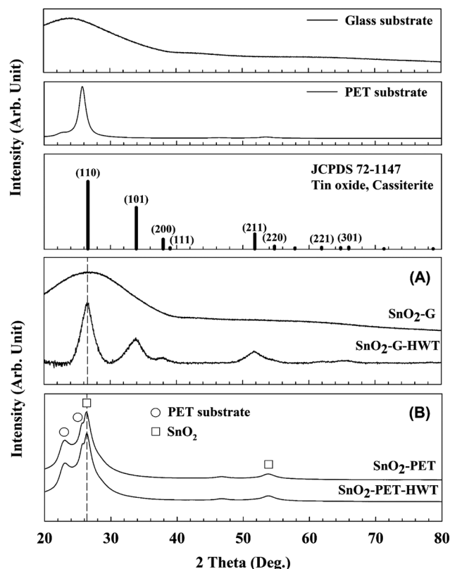
Fig. 8 The XRD patterns of SnO 2 (JCPDS 72-1147), the glass and PET substrate. (A) XRD patterns of the glass substrate and SnO 2 -G before and after the HWT process, (B) XRD patterns of the SnO 2 -PET before and after the HWT process.
