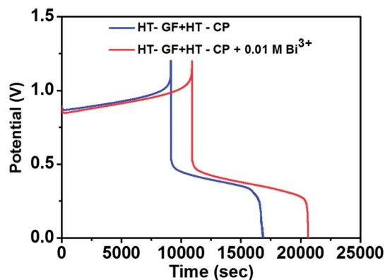
Fig. 7 Charge-discharge cycling curves of a Fe/Cu RFB with and without 0.01 M Bi 3+ in the electrolytes at a current density of 20 mA cm -2 .
