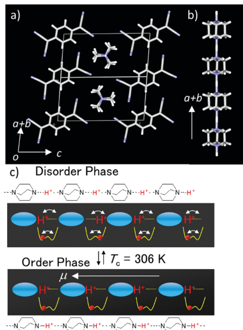
Fig. 3 Dynamic short-range collective proton transfer and dielectric switching in the organic semiconductor (\text{HDABCO}^+)\cdot 2(\text{TCNQ})_3 . (a) Unit cell viewed along the 1D (\text{N-H}^+\cdots\text{N})_\infty hydrogen-bonding chain and electrical conducting \pi -column of TCNQ. (b) High temperature 1D (\text{N-H}^+\cdots\text{N})_\infty hydrogen-bonding chain of \text{HDABCO}^+ cations along the a + b axis. Schematic potential energy curves of the \text{N-H}^+\cdots\text{N} hydrogen-bonding chain (c) at the high temperature paraelectric disordered phase (upper) and at the low temperature ordered ferroelectric phase (lower) for the proton orientation.
