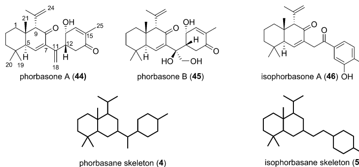
Fig. 6 The phorbasane and isophorbane natural products.
