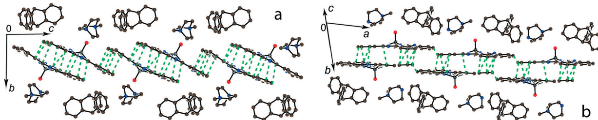
Fig. 11 View along the phthalocyanine layers composed of the \{Ti^{IV}(Pc^{3-})\}^-_2 dimers in 12 : view along the a (a) and approximately along the c (b) axes. Short van der Waal contacts between phthalocyanines are shown by green dashed lines.
