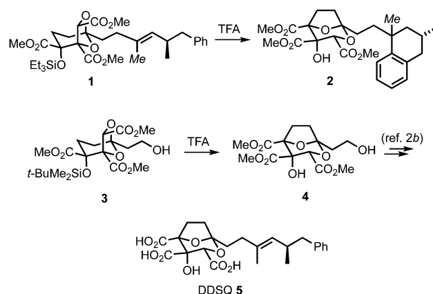
Scheme 1 Transketalisation approaches to (–)-6,7-dideoxysqualastatin H5.
