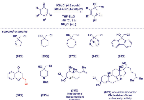
Scheme 10 Chemoselective addition of lithium carbenoids to α,β-unsaturated cyclic ketones.
