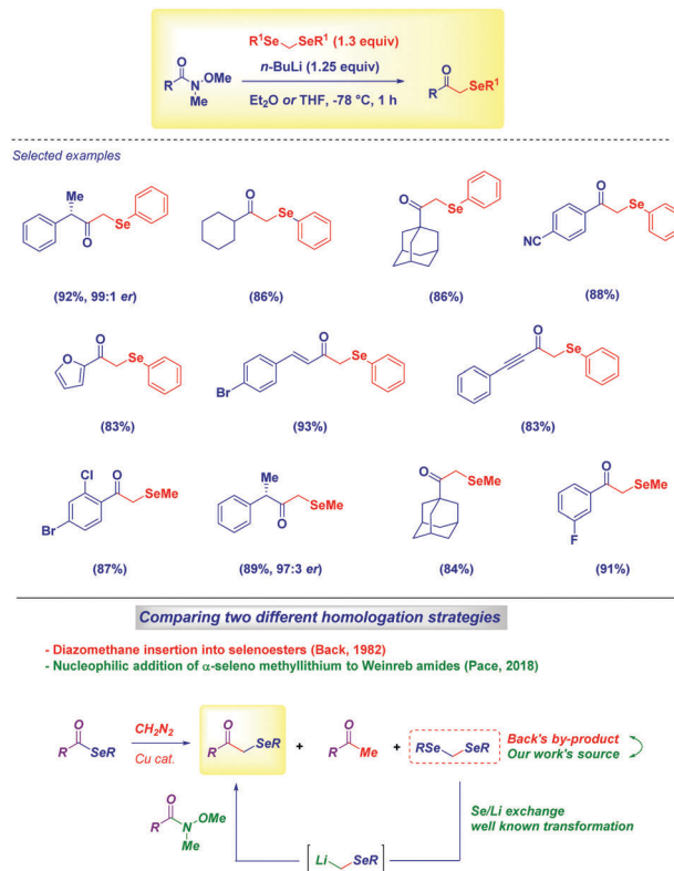
Scheme 9 Synthesis of α-seleno methylketones from Weinreb amides using diselenoacetals as precursors.
