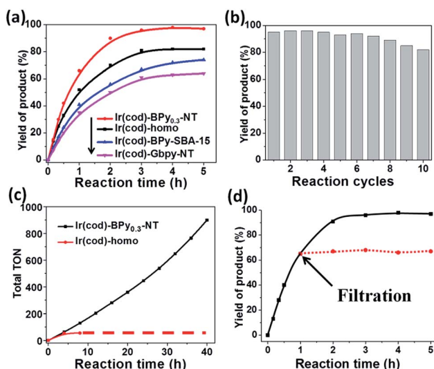
Fig. 6 (a) Reaction kinetic curves of benzene borylation catalyzed by Ir(cod)-homo (black line), Ir(cod)-BPY 0.3 -NT (red line), Ir(cod)-BPY-SBA-15 (blue line), and Ir(cod)-GbpY-NT (pink line). (b) Reusability of Ir(cod)-BPY 0.3 -NT for benzene borylation. (c) Total TONs of Ir(cod)-BPY 0.3 -NT (black line) and Ir(cod)-homo (red line) for the recycling. (d) Filtration experiment of Ir(cod)-BPY 0.3 -NT catalyst (red-dotted line).
