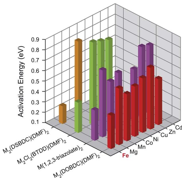
Fig. 3 Activation energies of M_2(\text{DOBDC})(\text{DMF})_2 , M_2(\text{DSBDC})(\text{DMF})_2 , M_2\text{Cl}_2(\text{BTDD})(\text{DMF})_2 , and M(1,2,3\text{-triazolate})_2 measured at 300–350 K, in vacuum, and in the dark.
