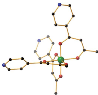
Fig. 1 The molecular structure of the fac -isomer of the metalloligand [M^{\text{III}}L_3] ( M = \text{Fe, Cr, Al} ). Colour code: M^{\text{III}} = \text{green} , \text{O} = \text{red} , \text{N} = \text{blue} , \text{C} = \text{black} . Hydrogen atoms have been omitted for clarity.
