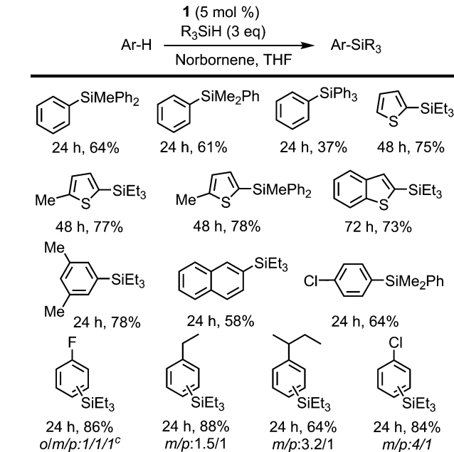
Scheme 3 Non-directed dehydrogenative silylation of aromatic and heteroaromatic rings. Reaction conditions: cat 1 (5 mol%), norbornene (0.40 mmol), arene (0.13 mmol), R 3 SiH (0.40 mmol) in THF (2 mL) at 110 °C. Isolated yields are shown. c Disilylated product was identified in 7% yield.
