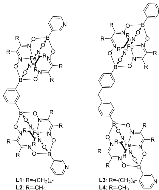
Fig. 1 The metalloligands L1–L4 .
