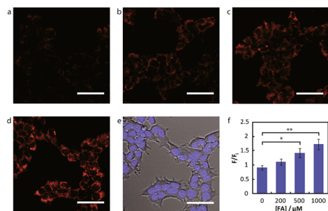
Fig. 11 Confocal microscopy of FA detection in living HEK293T cells using probe 7. Cells were treated with 10 \mu\text{M} probe 7 in BSS for 30 min at 37 °C, followed by an exchange with fresh BSS and addition of varying FA concentrations. Images are taken 30 min after addition of (a) vehicle, (b) 200 \mu\text{M} FA, (c) 500 \mu\text{M} FA, and (d) 1 mM FA. (e) Bright-field image of cells in (d) overlaid with image of 1 \mu\text{M} Hoechst 33342. Scale bar represents 50 \mu\text{m} in all images. (f) Mean fluorescence intensities of HEK293T cells treated with varying concentrations of FA for 30 min relative to mean fluorescence intensity before FA addition; error bars denote SEM (this figure has been adapted from ref. 61 with permission from ACS).
