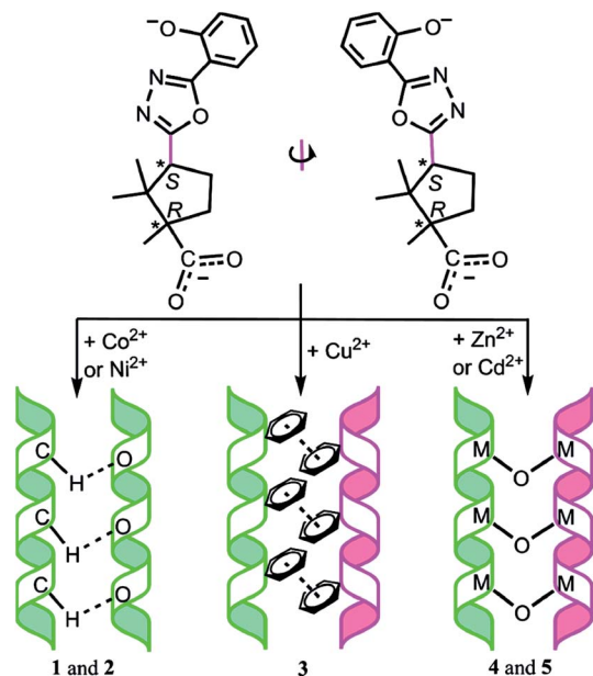
Scheme 15 Conformational twists of the asymmetric skeleton of (1R,3S)-1,2,2-trimethyl-3-((5-(2-hydroxy)phenyl-1,3,4-oxadiazol-2-yl)cyclopentanecarboxylic acid and different interhelical interactions in the prepared CPs. [Reprinted with permission from ref. 202. Copyright 2012, American Chemical Society.]
