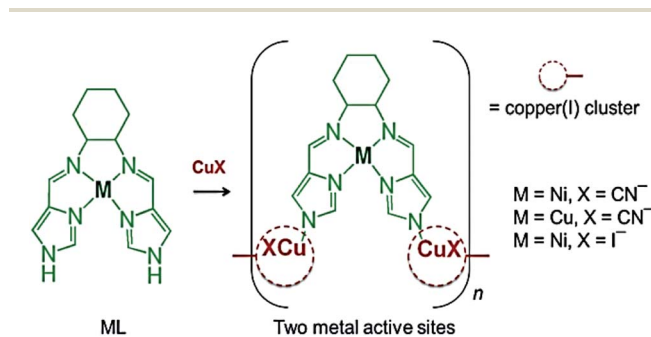
Scheme 3 Synthesis of \{[\text{NiL}]_2[\text{Cu(I)CN}]_9\}_n , \{[\text{Cu(II)L}]_2[\text{Cu(I)CN}]_9\}_n and \{[\text{NiL}][\text{Cu(I)I}]_2\}_n . [Reproduced from ref. 101 with permission from The Royal Society of Chemistry.]
