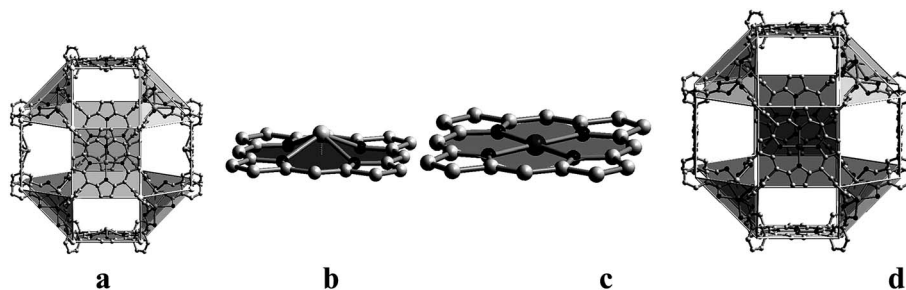
Fig. 27 (a) Representation of the crystal structure of the small cubucuboctahedron in MMPF-5 formed by 6 square Cd-Pp moieties and 8 triangular \text{Cd}(\text{CO}_2)_3 moieties. (b) The M-Pp macrocycle in MMPF-5, showing that the \text{Cd}(\text{II}) cation lies far out of the Pp plane. (c) The M-Pp macrocycle in MMPF-5(Co), showing that \text{Co}(\text{II}) cation is located within the plane of the Pp. (d) The small cubucuboctahedron in MMPF-5(Co) formed by 6 square Co-Pp moieties and 8 triangular \text{Cd}(\text{CO}_2)_3 moieties. [Reprinted with permission from ref. 60. Copyright 2013, Wiley-VCH Verlag GmbH & Co. KGaA, Weinheim.]
