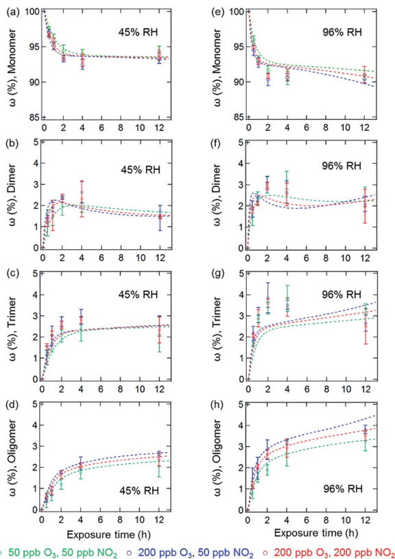
Fig. 2 Temporal evolution of protein oligomer mass fractions ( \omega (%), monomer, dimer, trimer and oligomer ( n \geq 4 )) upon exposure of BSA films (thickness 34 nm) to various O_3 / NO_2 concentrations: ((a)–(d)) at 45% RH; ((e)–(h)) at 96% RH. The data points and error bars represent the arithmetic mean values and standard deviations of duplicate experiments. The dashed lines are the results of the kinetic model.
