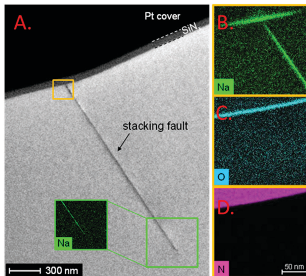
Fig. 5 (A) A bright-field TEM image of a stacking fault representing a single PID-shunt. (B–D) EDX mappings acquired in the STEM mode at the same stacking fault near the interface between Si and Si N x . A Na-EDX map of the lower part of the stacking fault is also shown in the inset of A. Reprint from ref. 65. Copyright 2014, Elsevier.
