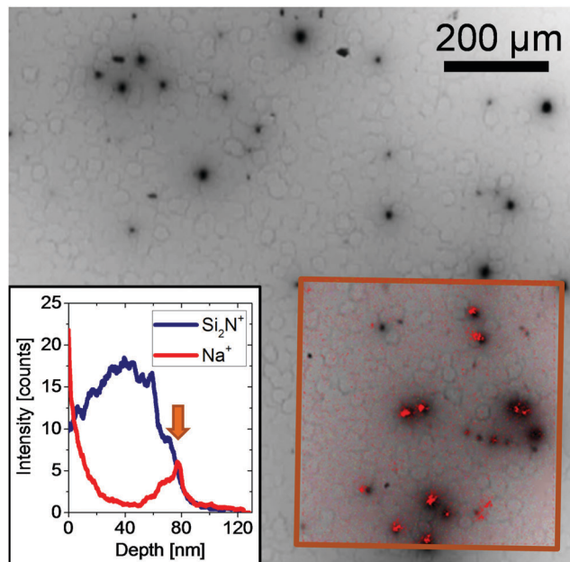
Fig. 4 An EBIC image of a monocrystalline silicon cell region with a high density of PID shunts acquired at an acceleration voltage of 30 kV. The inset shows the distribution of Na at the Si N x /Si interface measured by the ToF-SIMS. Reprint from ref. 65. Copyright 2014, Elsevier.
