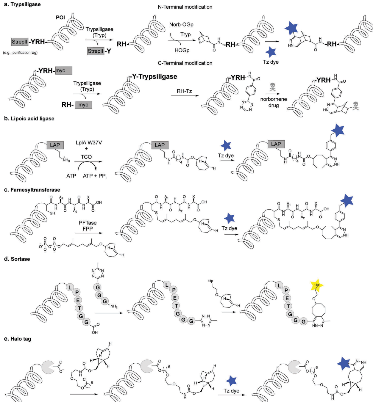
Fig. 27 Enzymatic methods for protein labelling through IEDDA. (a) Protein modification via trypsinylase. (b) Site-specific fluorescence labelling of proteins using LpIA and tetrazine reactions. (c) Labelling of CaaX peptide motif at the C-terminus with farnesyl isoprenoid analogs catalysed by PFTase. (d) Sortase bioconjugation. (e) HaloTag-based bioconjugation.
