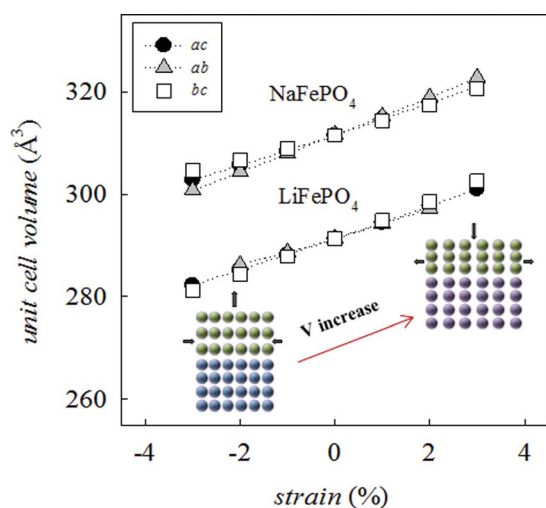
Fig. 2 Change in the calculated unit cell volume as a function of strain for \text{LiFePO}_4 and \text{NaFePO}_4 together with a schematic representation of the effect of compressive (<0%) or tensile (>0%) lattice strain on the thin film system.
