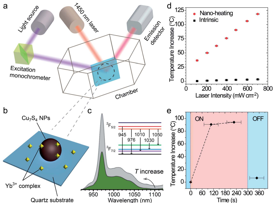
Fig. 3 (a) Schematic depiction of a surface temperature measurement of \text{Cu}_7\text{S}_4 nanostructures based on temperature-sensitive fluorescent molecules. The 410 nm laser was used to excite the fluorescent molecule and a 1450 nm laser was used as the heating source. (b) Magnified diagram of the testing sample on the quartz substrate. The ytterbium(III) complex was absorbed on the surface of \text{Cu}_7\text{S}_4 NPs as a temperature sensor. (c) T-Dependent luminescence spectra of the \text{Yb}^{3+} complex, with the inset showing the energy level corresponding to the luminescent wavelength. (d) Surface temperature increase ( \Delta T ) of \text{Cu}_7\text{S}_4 NPs (circle) and the sensor (square) at different intensities of 1450 nm laser illumination for 1 min. (e) On/off response of the surface temperature increase of \text{Cu}_7\text{S}_4 NPs.
