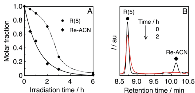
Fig. 6 (A) Residual R(5) and Re-ACN in solution during the photocatalytic reaction, obtained using UPLC analysis (Fig. S9, ESI † ). (B) UPLC chart of the photocatalytic system R(5)/Re-ACN before and after 2 h of irradiation; \lambda_{\text{det}} = 350 \text{ nm} .
