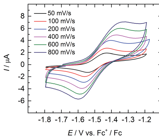
Fig. 5 Quasi-reversible oxidation wave of 3 at different scan rates. Measurement conducted in THF with \sim 0.1 \text{ M} [\text{N}(n\text{-Bu})_4][\text{BPh}_4] electrolyte, using \text{Fc}^+/\text{Fc} couple as internal standard.
