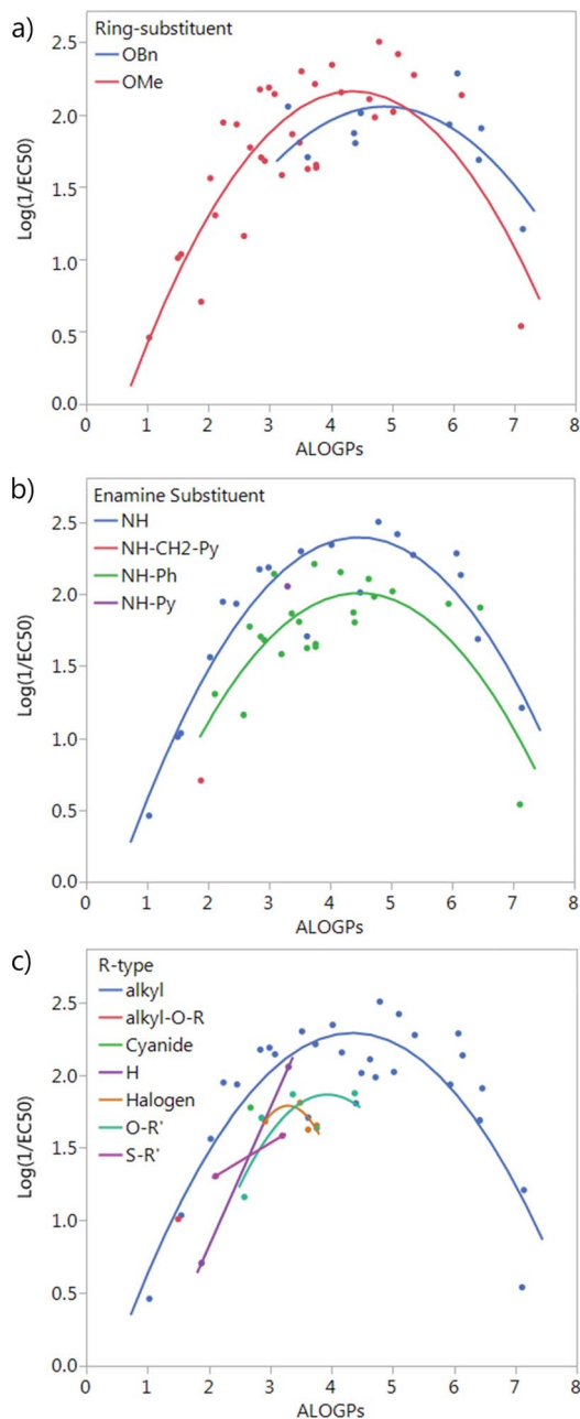
Fig. 4 Plot of \log(1/\text{EC}_{50}) vs. \text{ALOGPs} splitting the dataset by different substituents: (a) ring-substituent ( R_4 ), (b) enamine-substituent ( R_5 ), (c) R-type ( R_6 ), see Fig. 3.
