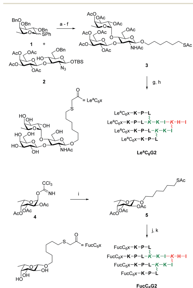
Scheme 2 Synthesis of Le a C 6 G2 and FucC 6 G2 . Conditions: (a) N -Iodosuccinimide, AgOTf, CH 2 Cl 2 , 0 °C, 30 min (quant.); (b) H 2 , Pd(OH) 2 , THF, AcOH, 17 h, 25 °C; (c) pyridine/Ac 2 O, cat. DMAP/NMM, CH 2 Cl 2 , 25 °C, 4 h (55% over 2 steps); (d) TBAF, AcOH, 25 °C, 17 h (60%); (e) Cl 3 CCN, DBU, CH 2 Cl 2 , 0 °C, 40 min (80%); (f) AcS(CH 2 ) 6 OH, TMSOTf, CH 2 Cl 2 , 0 °C, 20 min (64%); (g) K 2 CO 3 , MeOH, 25 °C, 1 h (75%); (h) ClAcD2 , KI, DIPEA, H 2 O/CH 3 CN, 25 °C, 17 h, then prep. HPLC (63%); (i) step g (84%); (j) step f (75%); (k) step h (31%). See ESI† for synthesis details.
