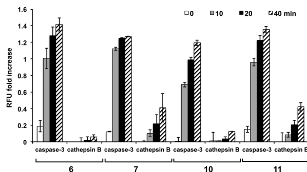
Fig. 3 Comparison of activation by caspase-3 (15 nM) and cathepsin B (25 nM) with substrates (10 \mu\text{M} , n = 3 ) containing proline or valine at the X_2 position ( 6 vs. 7 and 10 vs. 11 ). The fluorescence was divided by the background fluorescence (no enzyme) to give a "RFU fold increase" for each probe ( (\text{RFU}_{\text{enzyme}}/\text{RFU}_{\text{blank}}) - 1 ). This was done to allow comparison with the reduced fluorescence of fluorescein in the acidic cathepsin buffer (pH 5).
