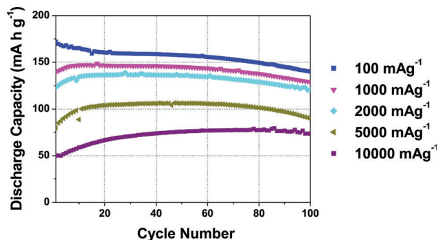
Fig. 3 Cycling performance of the 5% Mg-doped \text{Na}_{2/3}\text{Mn}_{0.95}\text{Mg}_{0.05}\text{O}_2 cathode, evaluated at various discharge rates. The cells were cycled between 1.5 and 4.0 V vs. \text{Na}^+/\text{Na} , charged at 13 \text{ mA g}^{-1} and discharged at various rates, as indicated.
