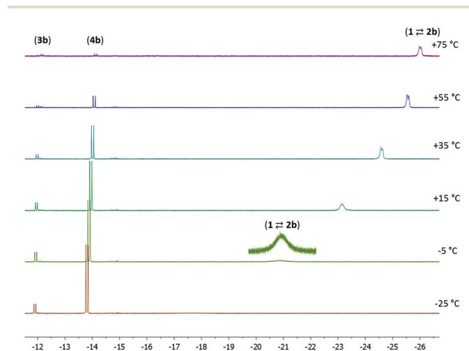
Fig. 3 Variable temperature NMR spectra for the reaction between 1 and 4-pentenenitrile (1 : 1, 0.04 M solution in toluene- d_8 ).
