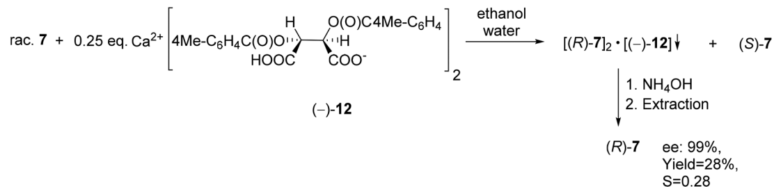
Scheme 16 The resolution of 4-chloro-5-methyl-1-phenyl-1,2,3,6-tetrahydrophosphinine 1-oxide (7) with \text{Ca}(\text{H-DPTTA})_2 [(-)-12].
