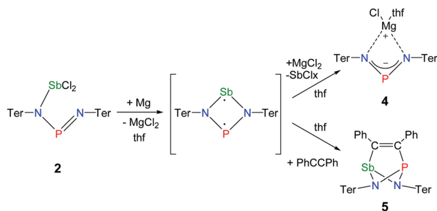
Fig. 8 Reduction of 2 with magnesium and trapping of the transient biradical.
